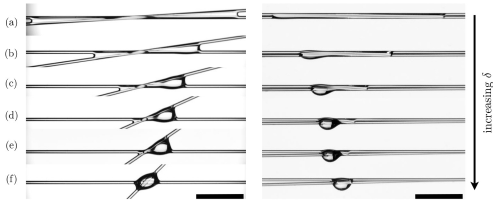
Fig. 3. Evolution of the morphology of a drop of volume V = 2 \mu\ell of silicone oil (5 cSt) on two touching crossed fibers ( h = 0 ) of radius a = 150 \mu\text{m} as the angle \delta between the fibers is varied: top (left) and side (right) views. The liquid starts in a column state for a small tilting angle, (a) \delta = 4^\circ . As the angle is increased, a mixed morphology is observed: (b) \delta = 9^\circ , (c) \delta = 15^\circ , (d) \delta = 25^\circ and (e) \delta = 35^\circ . Finally, at larger angles, (f) \delta = 45^\circ , a drop lies at the crossing point of the fibers. Scale bars are 5 mm.
