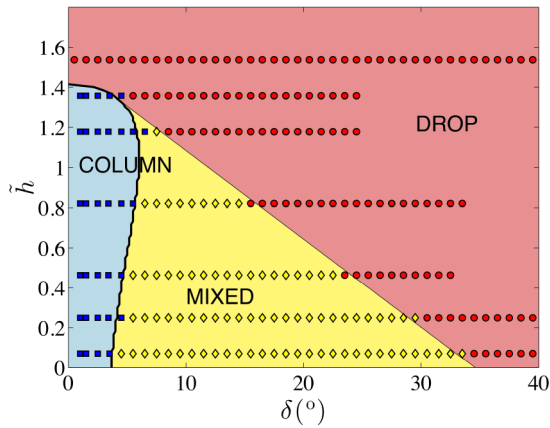
Fig. 8. Morphology diagram for a drop of silicone oil places on separated crossed fibers of radii a = 150 \mu\text{m} in the parameter space (\delta, \tilde{h}) using a volume \tilde{V} = 592 of silicone oil ( \theta_E = 0^\circ ). Red circles show the drop morphology, blue squares the column morphology and yellow diamonds are the mixed morphology. The thick solid line is the prediction of our model.
