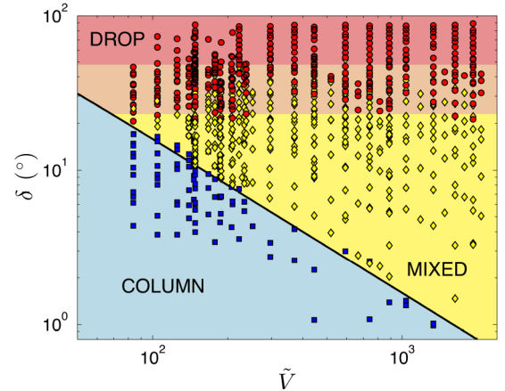
Fig. 11. Morphology diagram for the touching crossed fibers ( h = 0 ) in the parameter space ( \tilde{V} , \delta ). Red circles show the drop morphology, blue squares the column morphology and yellow diamonds are the mixed morphology. The light orange region corresponds to the region where both column and mixed morphologies are observed. The solid black line corresponds to the analytical prediction of the maximum angle where the column state is possible for a given volume \tilde{V} .
