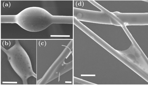
Fig. 1. SEM pictures of drops of binder lying on glass wool. (a) Drop on a single fiber, (b) liquid in the drop state between two crossed fibers, (c) and (d) liquid in the column state between two fibers. Scale bars are 10\ \mu\text{m} (pictures from Saint-Gobain Research, reproduced with permission from Bintein [21]).
