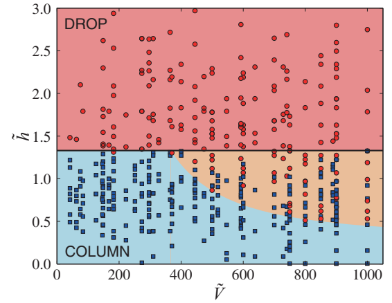
Fig. 10. Morphology diagram in the parameter space ( \tilde{V} , \tilde{h} ) using a partially wetting liquid (dodecane) on parallel fibers of radii a = [100, 150, 230] \mu\text{m} and a volume of liquid V \in [0.5, 4] \mu\text{l} . Red circles show the drop morphologies and blue squares the column morphology. The light orange region corresponds to the region where both morphology are observed. The horizontal solid line corresponds to the analytical prediction for dodecane: \tilde{h}_{\text{max}} \simeq 1.33 .
