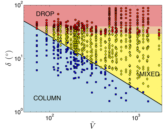
Fig. 7. Morphology diagram for touching crossed fibers of radii a = [100, 150, 180, 230] \mu\text{m} in the parameter space (\tilde{V}, \delta) using a volume V \in [0.5, 7] \mu\text{l} of silicone oil ( \theta_E = 0^\circ ). Red circles show the drop morphology, blue squares the column morphology and yellow diamonds are the mixed morphology. The light orange region corresponds to the parameters where both drop and the mixed morphology are observed. The solid line corresponds to the theoretical maximum angle, for a given volume \tilde{V} , below which the column state is possible.
