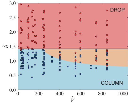
Fig. 6. Morphology diagram in the parameter space (\tilde{V}, \tilde{h}) using silicone oil ( \theta_E = 0^\circ ) on parallel fibers ( \delta = 0^\circ ) of radii a = [100, 150, 230] \mu\text{m} and a volume of liquid V \in [0.5, 4] \mu\text{l} . Red circles show the drop morphology and blue squares the column morphology. The light orange region corresponds to the region where both morphologies are observed. The horizontal solid line corresponds to the theoretical maximum separation distance where the column state is possible, \tilde{d}_{\text{max}} = \sqrt{2} .
