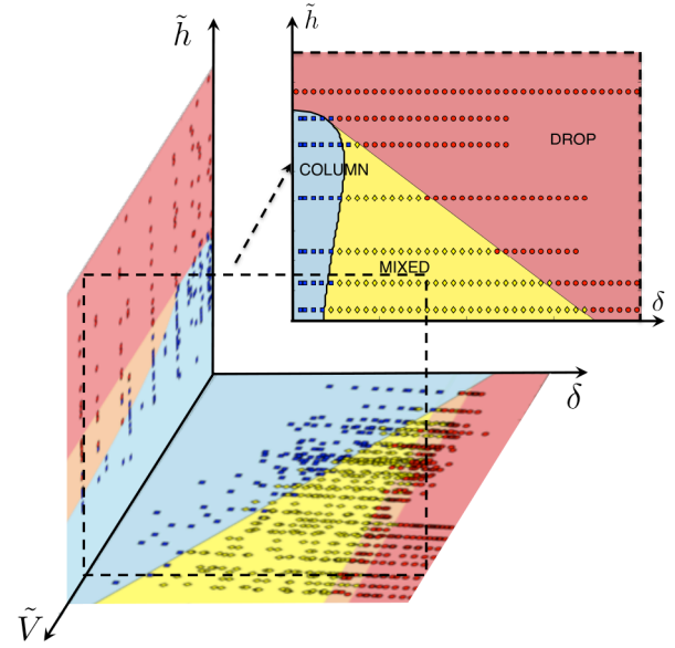
Fig. 9. Morphology diagram for a pair of fibers randomly oriented wetted by a drop of silicone oil ( \theta_E = 0^\circ ) in the parameter space (\tilde{V}, \delta, \tilde{h}) . Red circles show the drop morphology, blue squares the column morphology and yellow diamonds are the mixed morphology. The light orange region corresponds to the region where both morphologies are observed.
